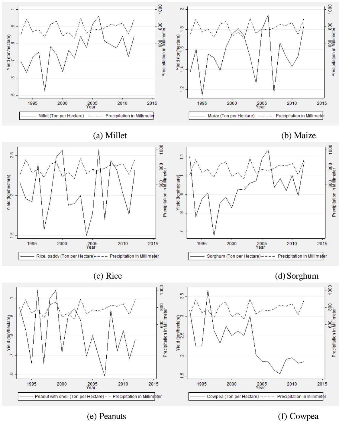
Figure 1: Yield of major commodities (tone per hectare) and rainfall (Meter) in Burkina Faso from 1994 to 2014.
